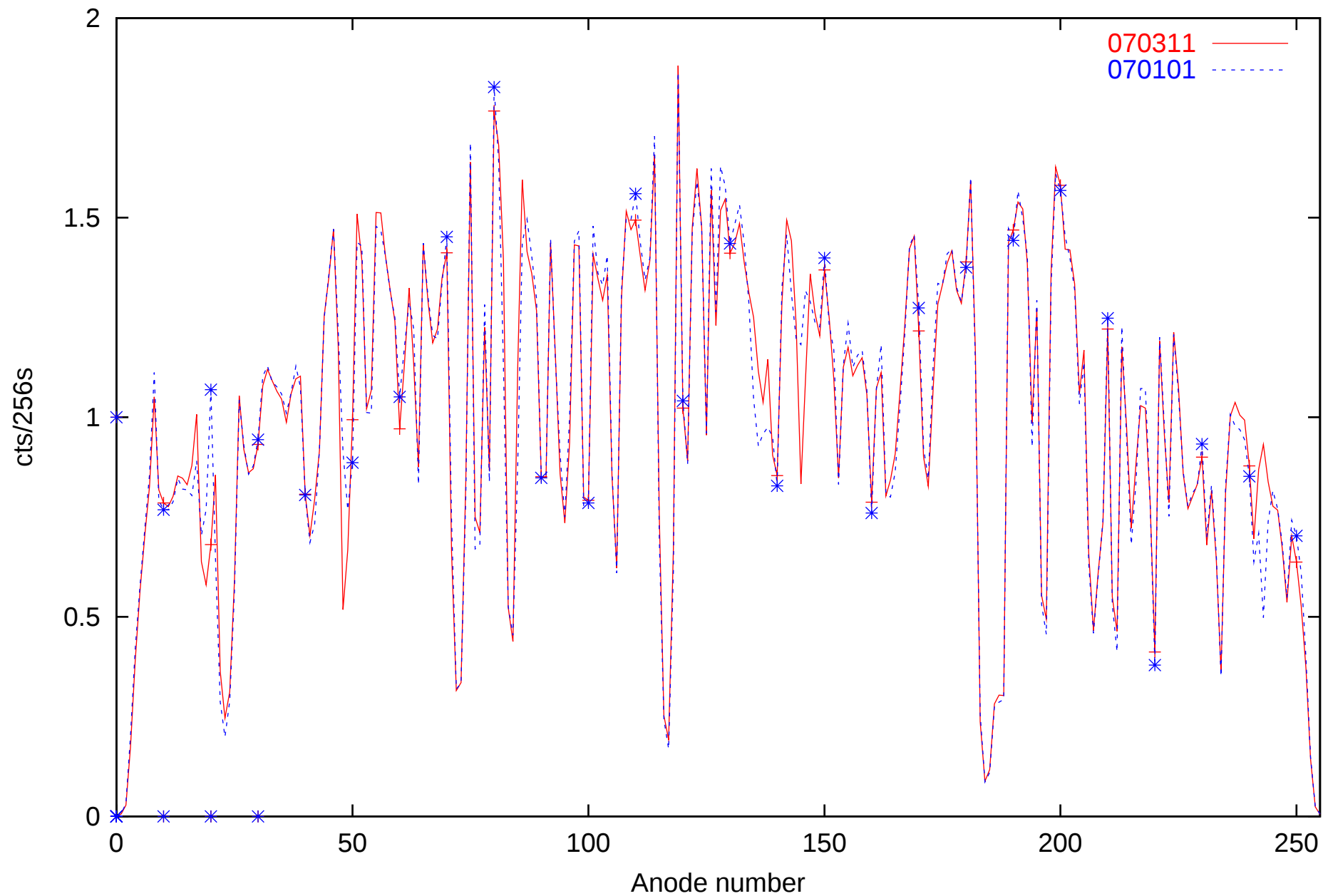
JEM-X1 anode counts
