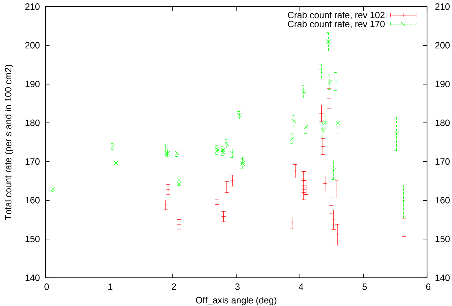
CRAB flux determinations. JEM-X1
