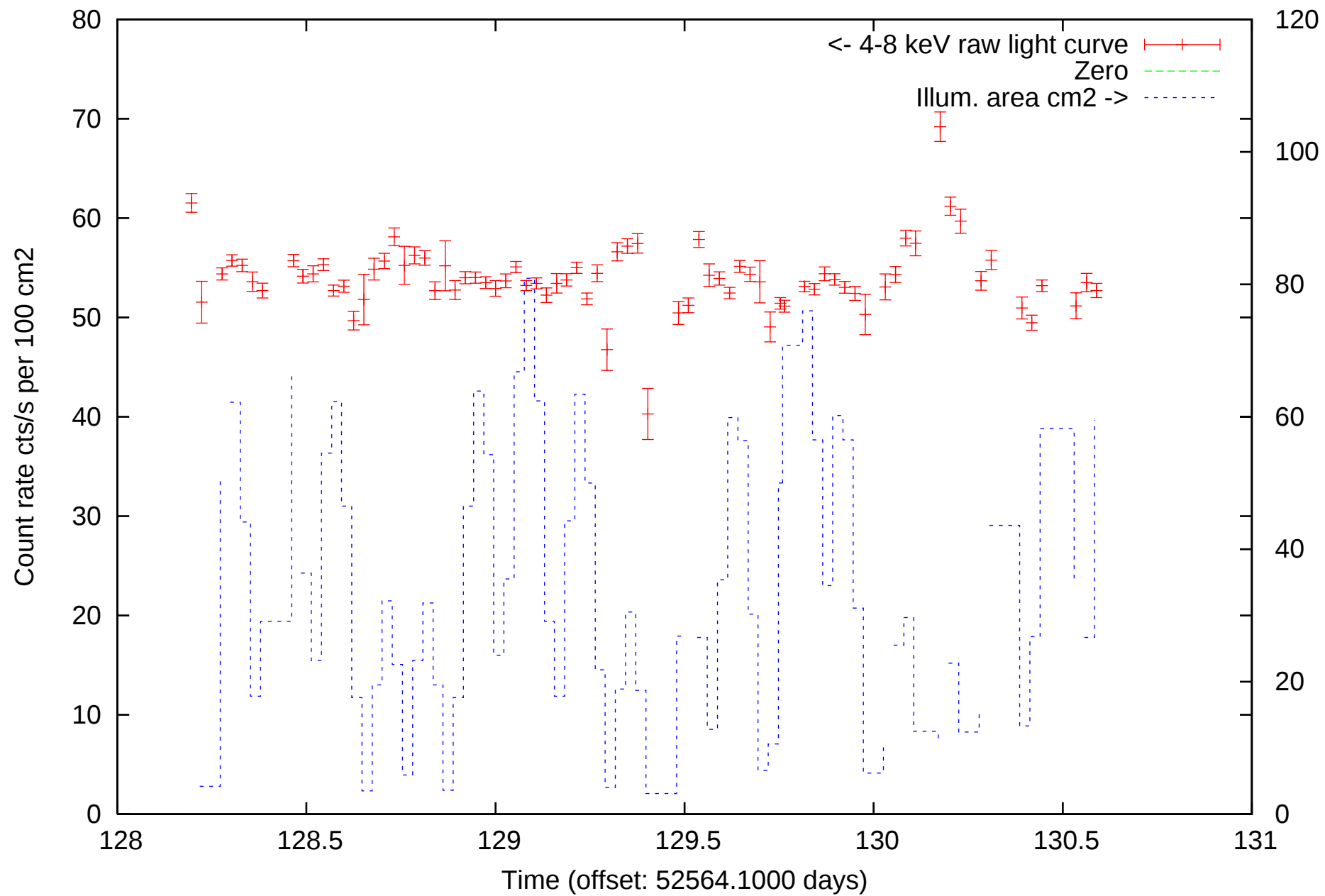
CRAB light curve, time_bin: 2200.0 s (JEM-X1)
